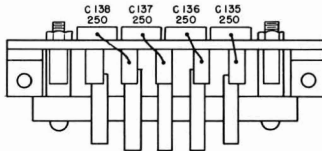
Pulse Forming Line RB5
