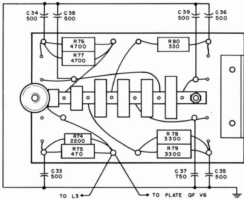
Pulse Forming Line RB5
