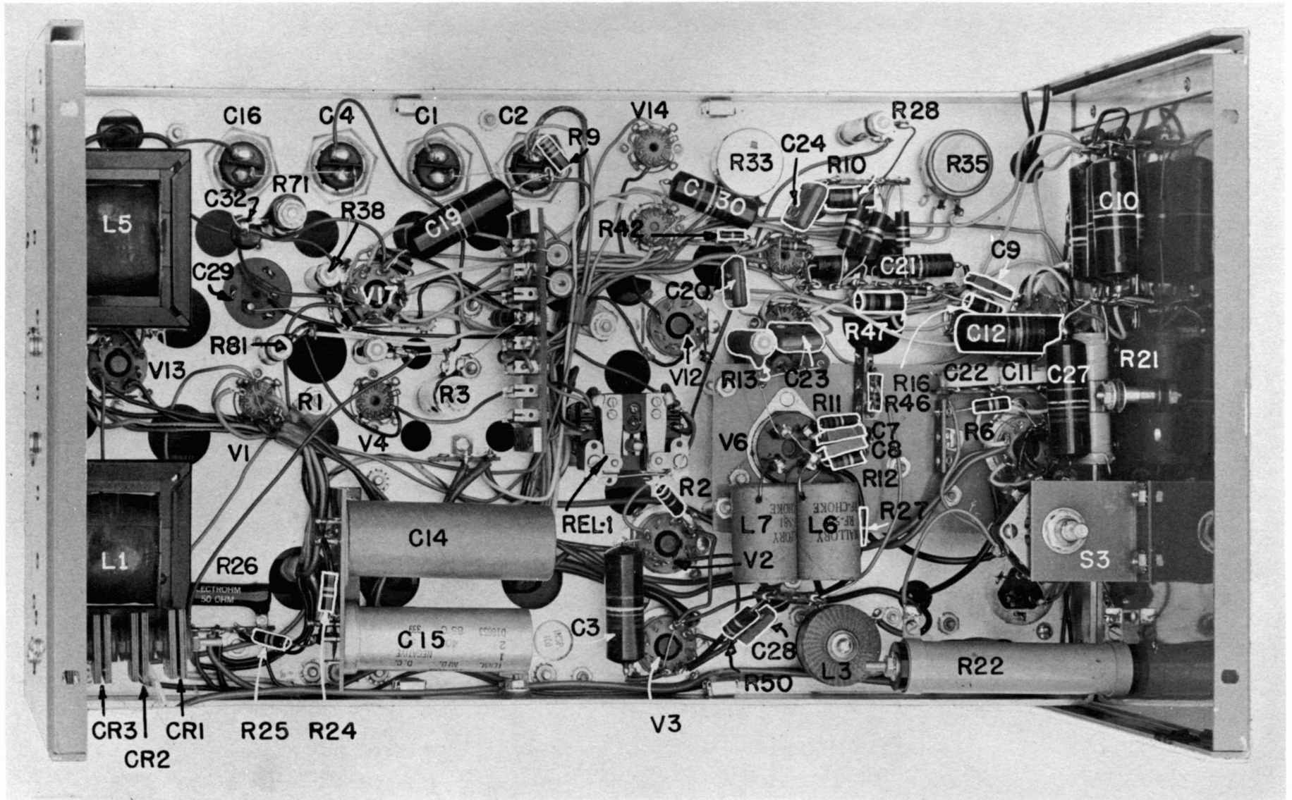
Fig. 4-3 Pulse Generator, Typical Front View of Power Supply and Pulse Generating Sections (Removed)
