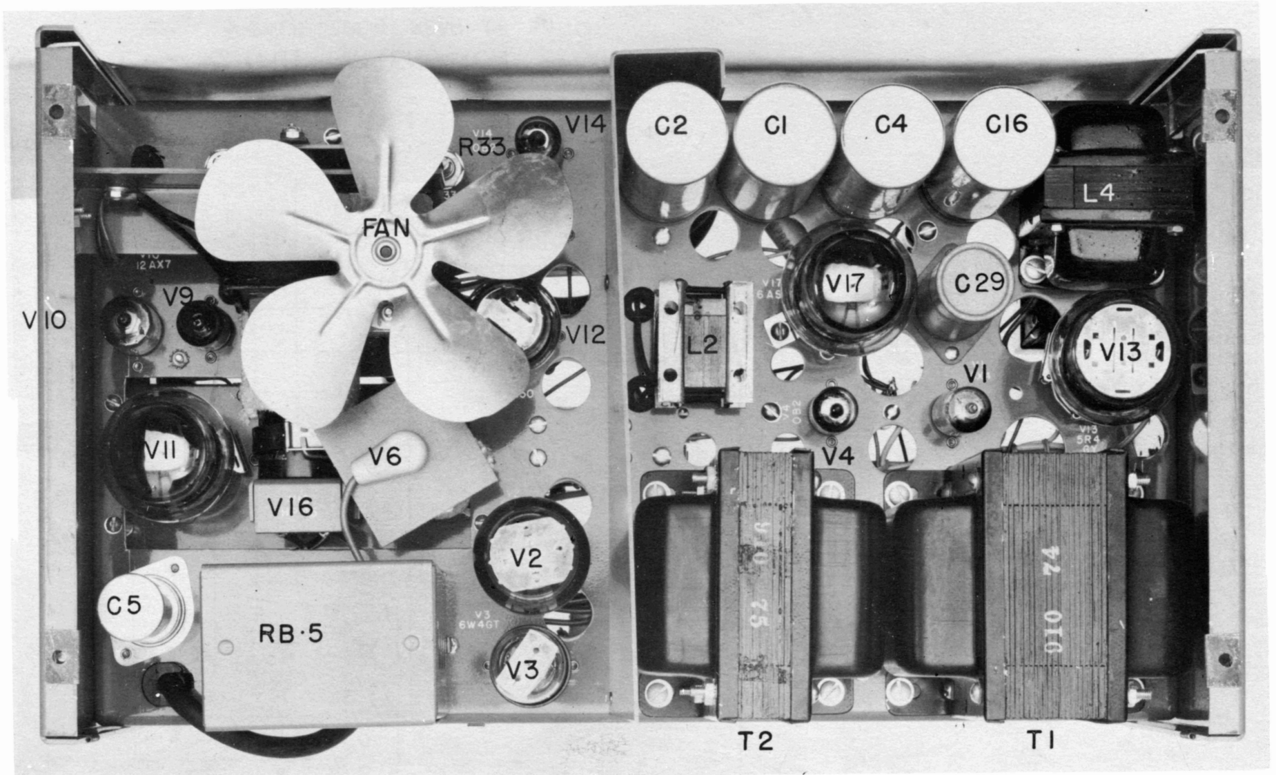
Fig. 4-4 Pulse Generator, Typical Rear View of Power Supply and Pulse Generating Sections (Removed)
